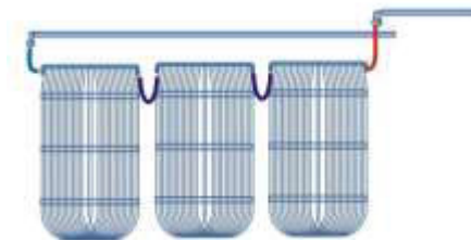
Series connection when flexible hoses are used
