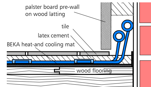
Variation B: Layout for modernizing
