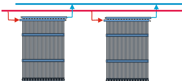
Parallel single connection to „Tichelmann“
