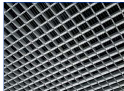
Nearly invisible: uncolored capillary tube mats unite with the open ceiling construction
